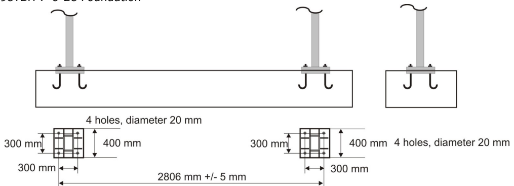
EP098TBH 7-6-28 Foundation
